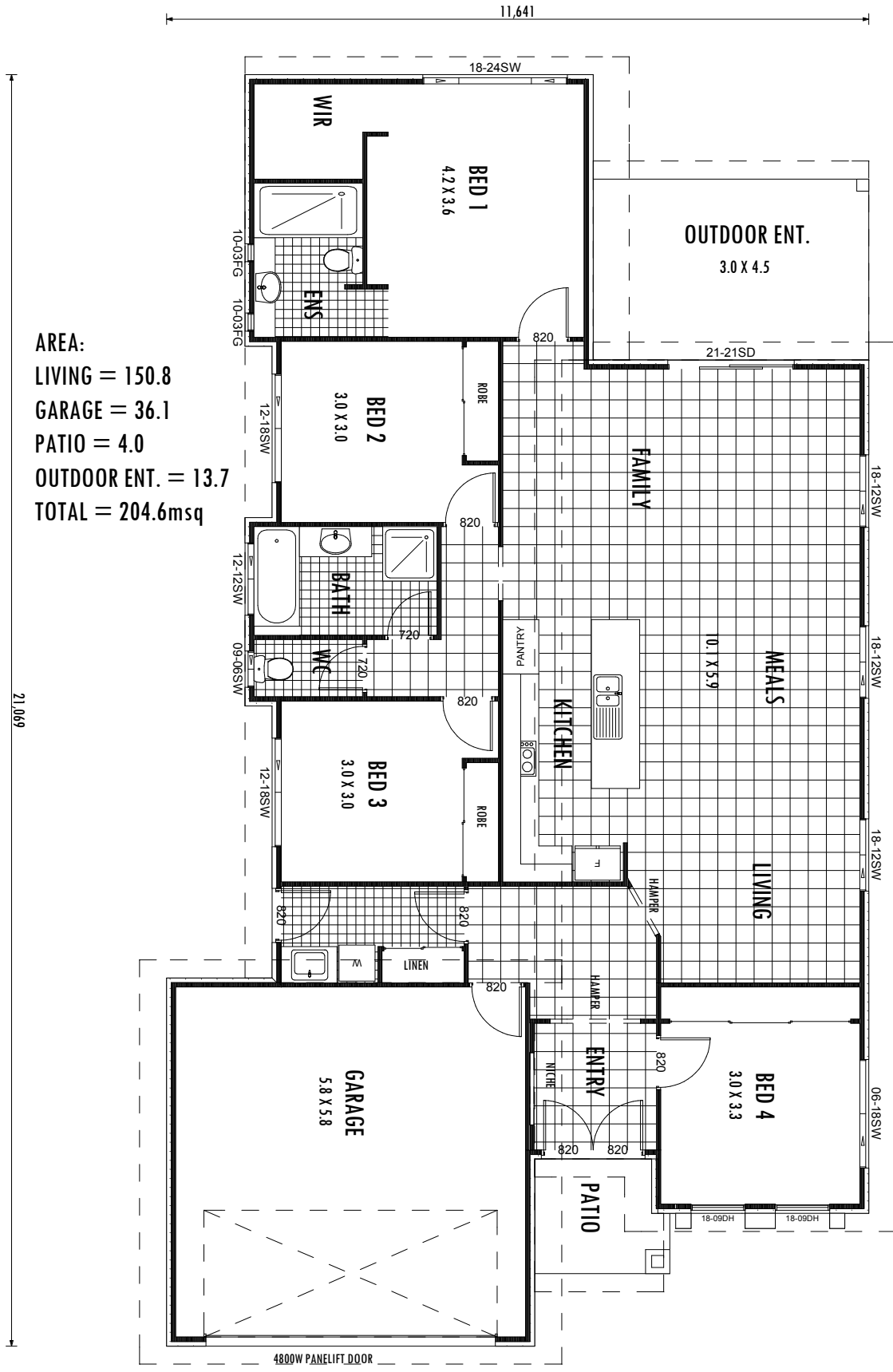
FLOOR PLAN
